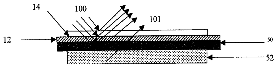
Fig. 7 (PRIOR ART)
