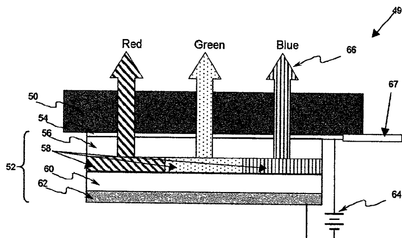
Fig. 5: (Prior art)
