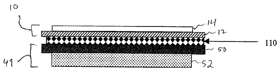
Fig. 8 (PRIOR ART)
